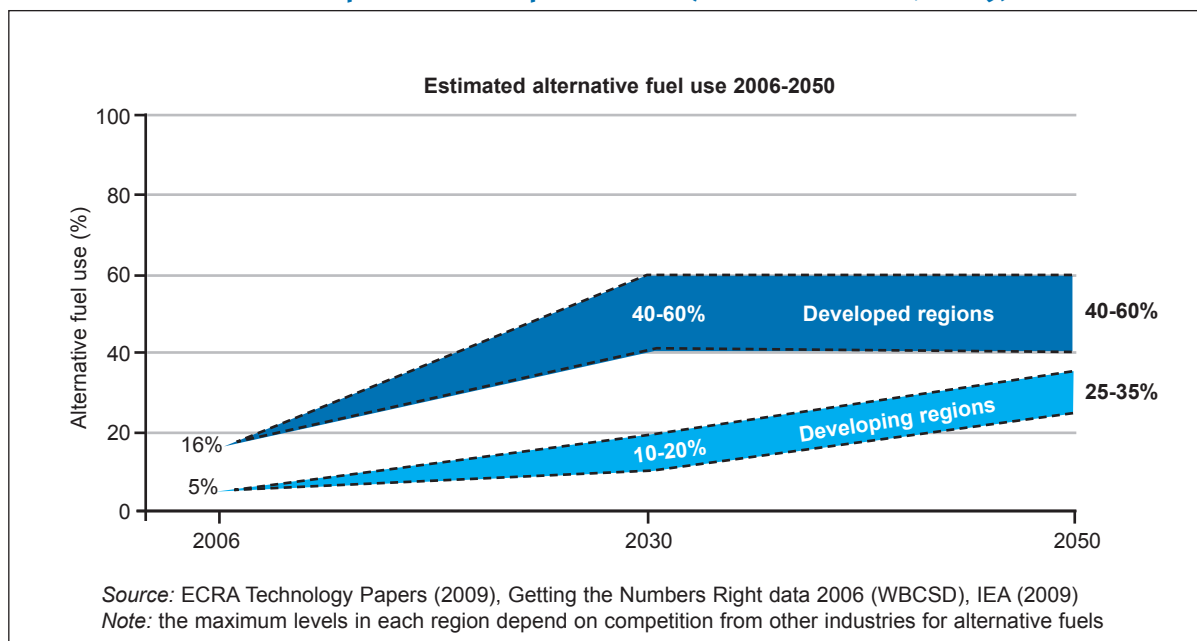
Figure 7 Alternative fuels roadmap for cement production (IEA and WBCSD, 2009)
