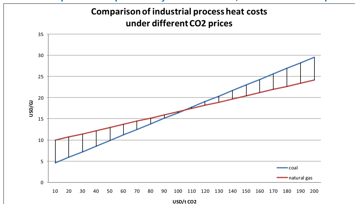
Cost of useful process heat produced by main fossil fuels, under different CO 2 prices
