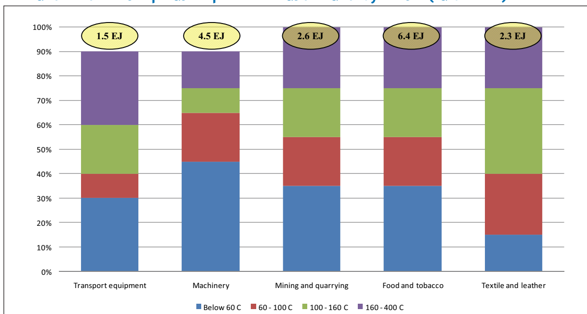
Figure 10 Low and medium temperature process heat demand by sector (Taibi 2010)
