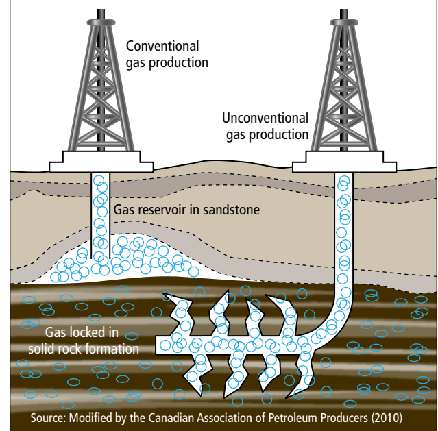
FIGURE 1 Shale Gas Extraction Technology
