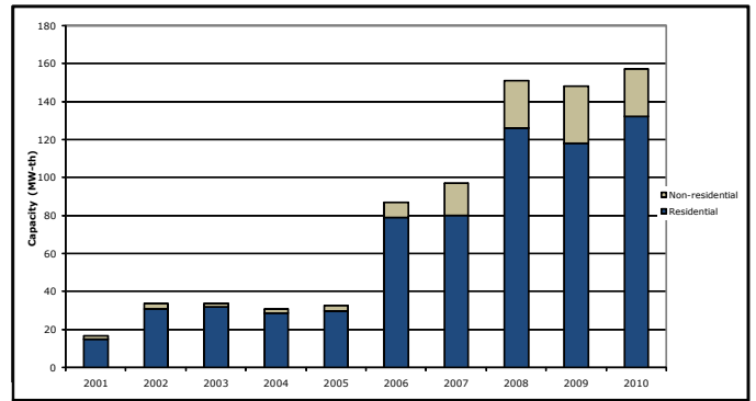
Figure 7: Annual Installed U.S. Capacity for Solar Heating and Cooling (2001-2010)
