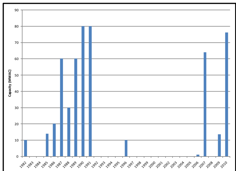
Figure 6: Annual Installed U.S. CSP Capacity (1982-2010)
