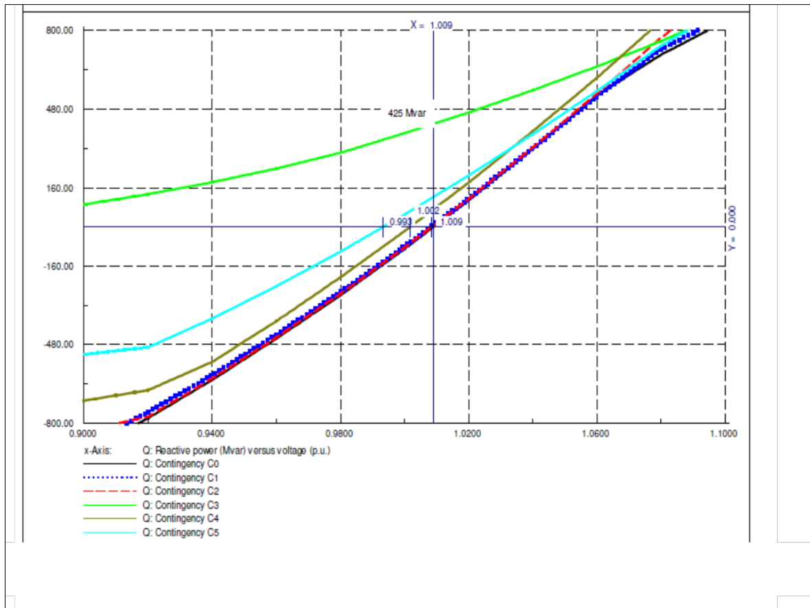
Figure 9 - QV-curves for various contingencies
