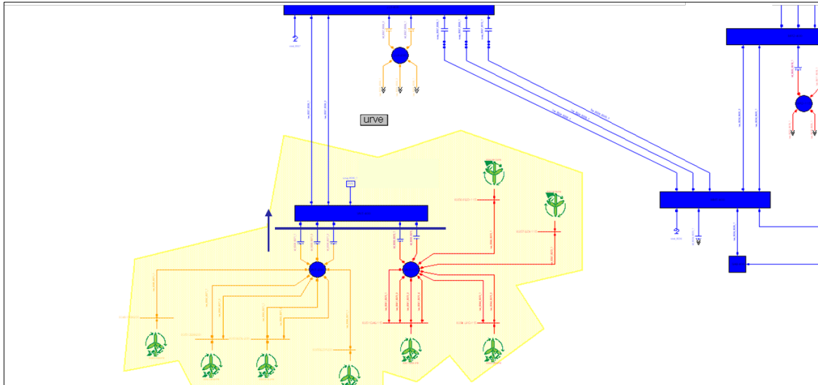
Figure 8 - Example for the connection of large wind farms to a transmission grid
