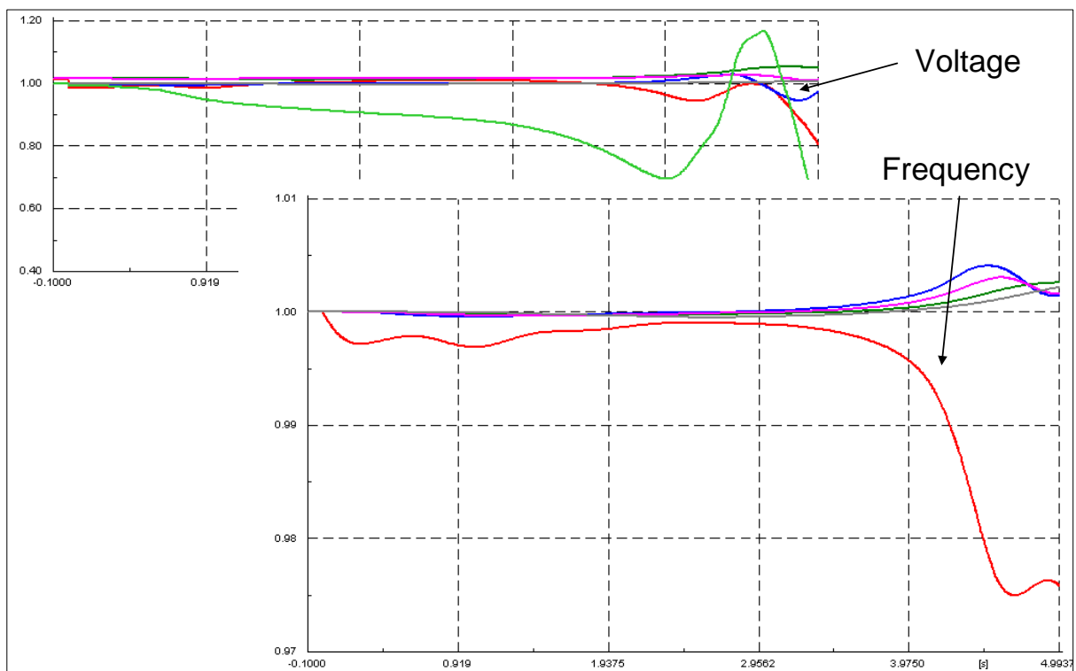
Figure 4: Voltage and frequency of a large generator leading to short-term voltage collapse
