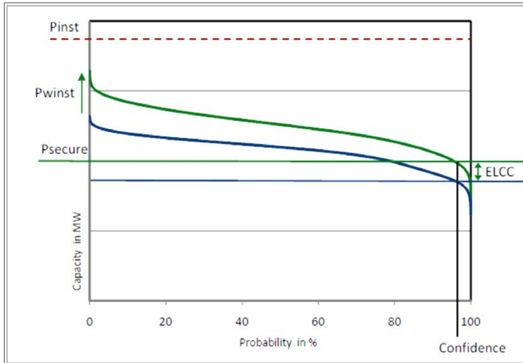
Figure 5: Definition of ELCC at a given confidence level
