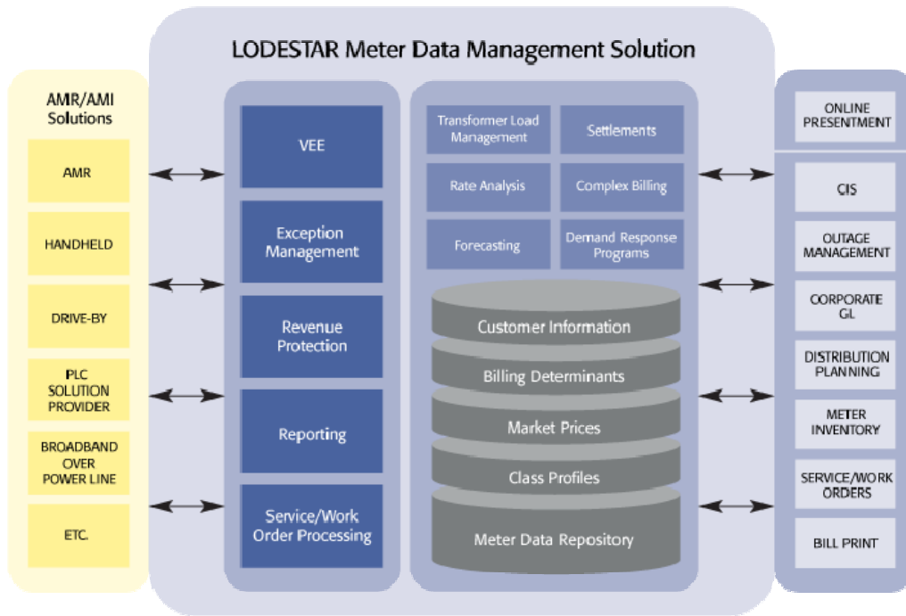
Figure 11: MDMS Concept
