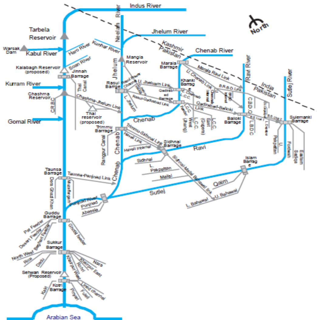
Figure 2—The Indus River basin and irrigation canals (Briscoe & Qamar, 2005b) as modeled in RWSM-Pak
