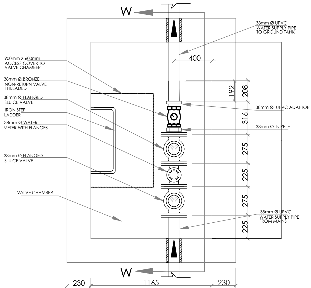
EXTERNAL WORKS: DETAILS OF WATER MAINS VALVE CHAMBER.
