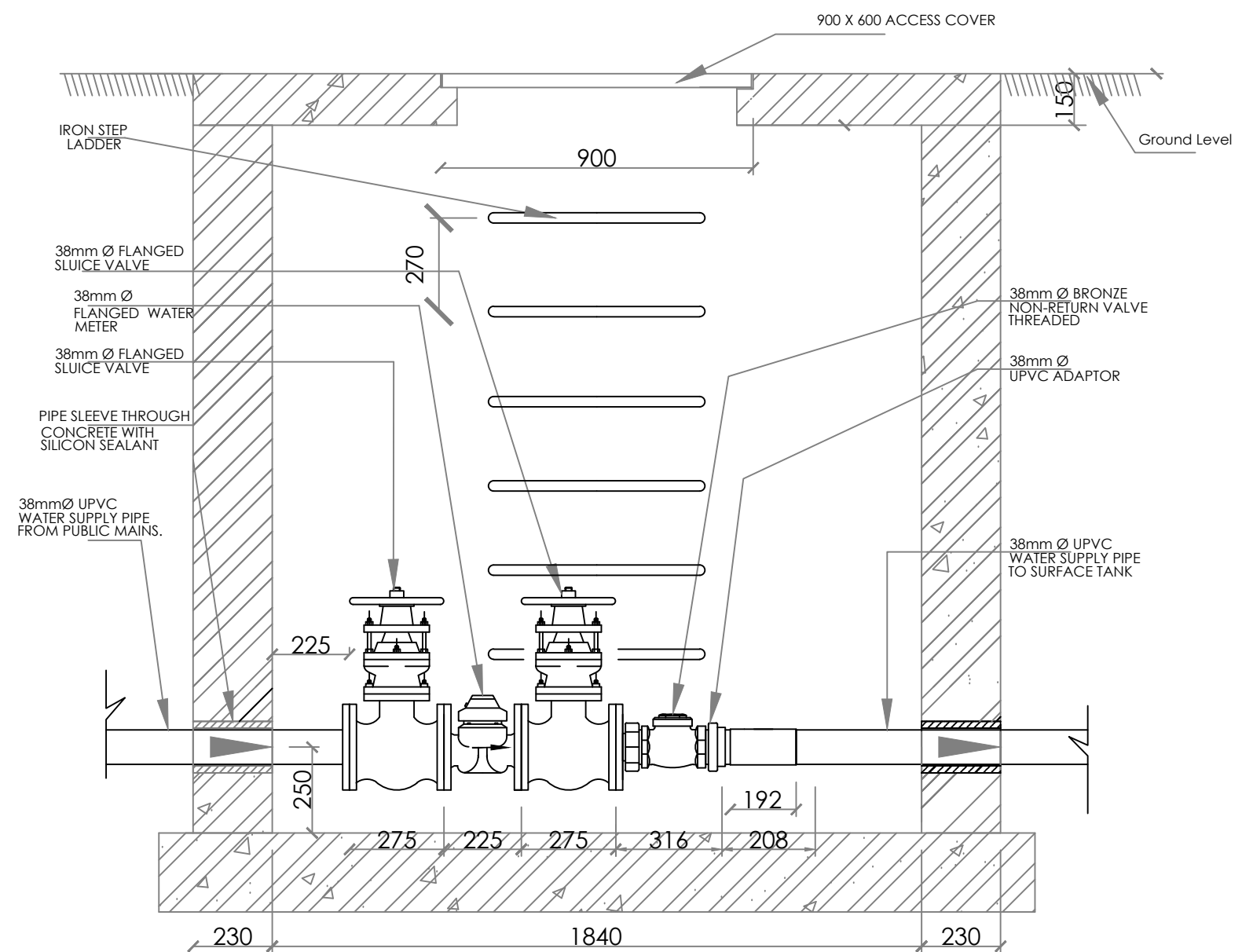
ELEVATION W-W: MAINS VALVE CHAMBER
