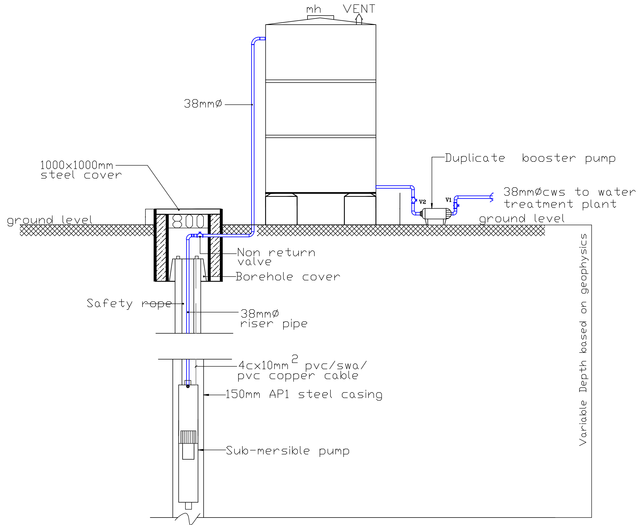
TYPICAL DETAIL OF GROUND WATER TANK
