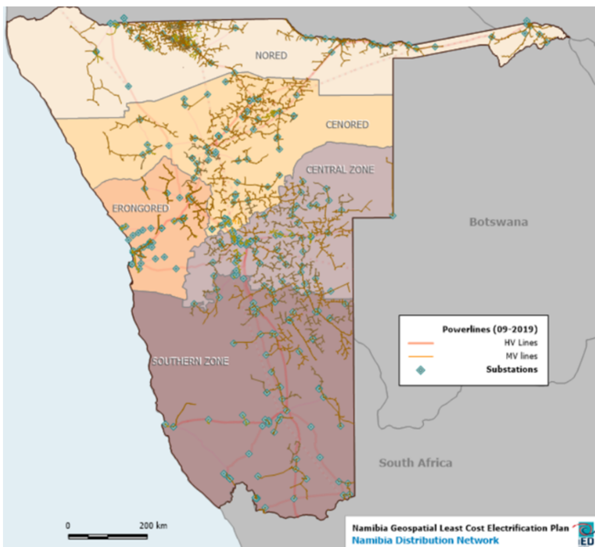
Figure 8: Distribution Network in Namibia. Image Source: Namibia: Geospatial Least Cost Electrification Plan, 2021
