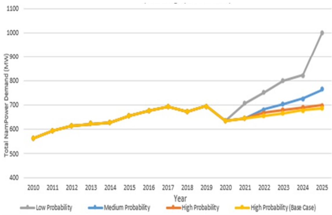
Figure 45: Namibia's electrical load forecast (including system losses). Image Source: NamPower
