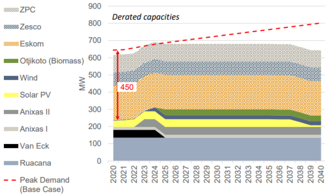
Figure 9: Power capacity supply and demand balance. Image Source: NIRP, 2021
