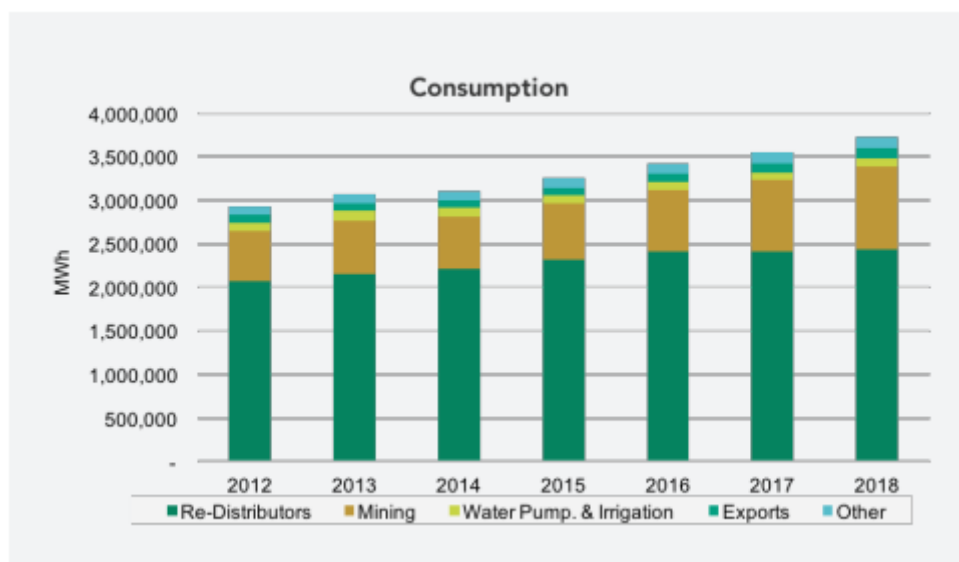
Figure 6: Consumption by customers groups (MWh). Image Source: NamPower, 2019
