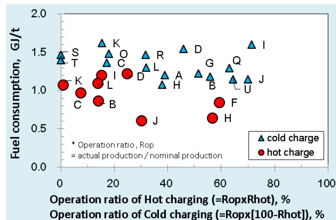
Figure 33: Effect of operation ratio for hot and cold charge on fuel consumption
